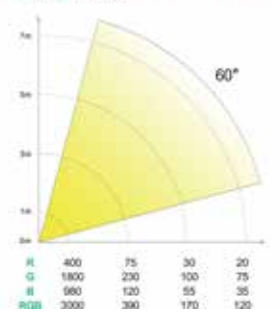
PHOTOMETRIC BEAM ANGLE DATA (FC=LUX x 0.0929)
